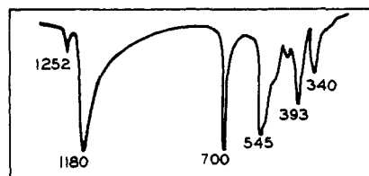
Figure 4. Infrared spectrum of C_7Cl_7^+Al_2Cl_7^- ( 3 ).
