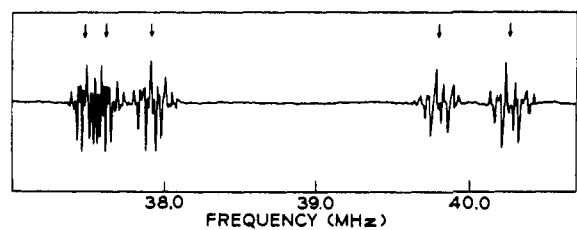
Figure 2. Nuclear quadrupole resonance spectrum of 1 at room temperature.
